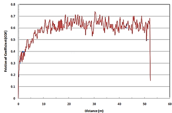
Fig. 10. Changes in the friction coefficient of the reference sample in wear under a load of 300 g force and a distance of 50 m.
