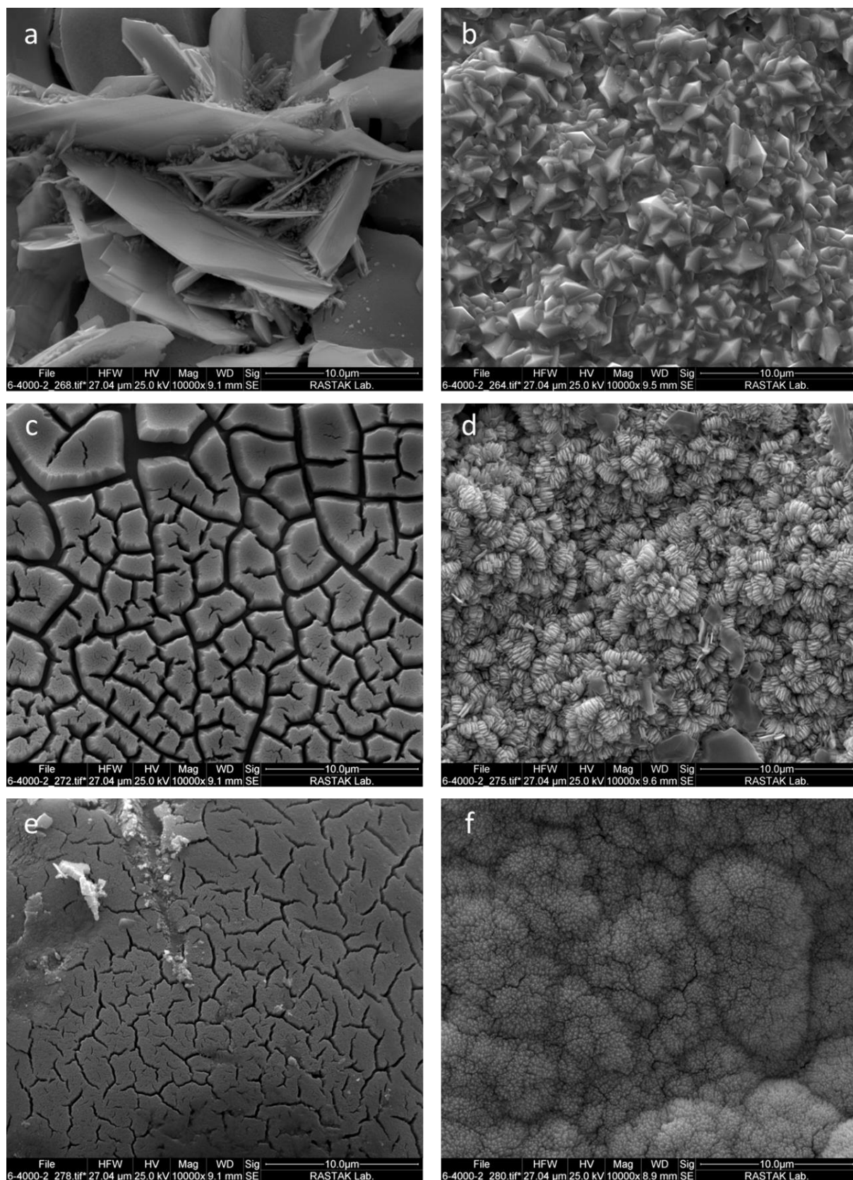
Fig. 4. SEM micrographs of samples electrodeposited in 0.1 M HNO 3 , 0.5 M Pb(NO 3 ) 2 and a) Sample A2, b) Sample B2, c) Sample C2, d) Sample C2 on Ti/ \alpha -PbO 2 , e) Sample D2, f) Sample E2
