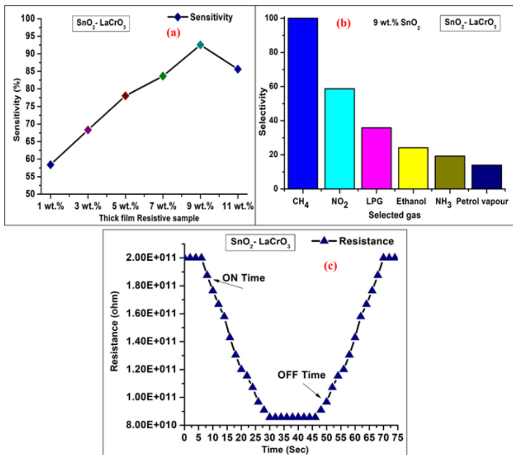
Fig. 12. Plot of a) sensitivity versus wt.% SnO 2 additive b) selectivity histogram of 9 wt.% SnO 2 added LaCrO 3 thick films c) response and recovery time plot of 9 wt.% SnO 2 added LaCrO 3 thick films
