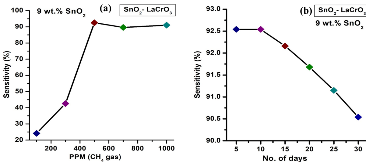
Fig. 13. Plot of a) sensitivity versus \text{CH}_4 gas concentration in ppm b) Reproducibility graph for \text{CH}_4 gas of 9 wt.% SnO 2 added LaCrO 3 thick films
