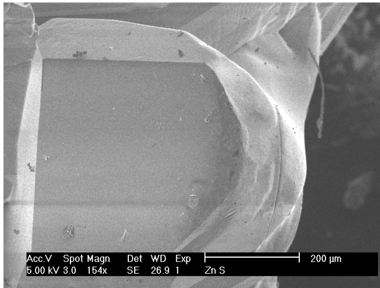
Fig. 5. ZnS single crystal in platelet form grown at 1002 °C.
